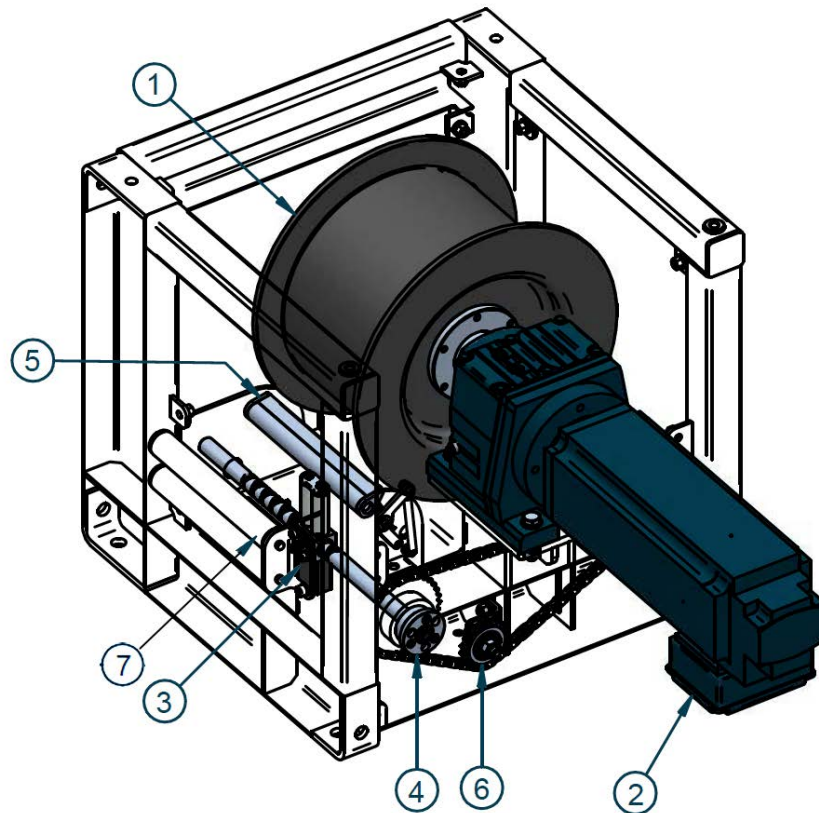
Drum unit, transparent view
