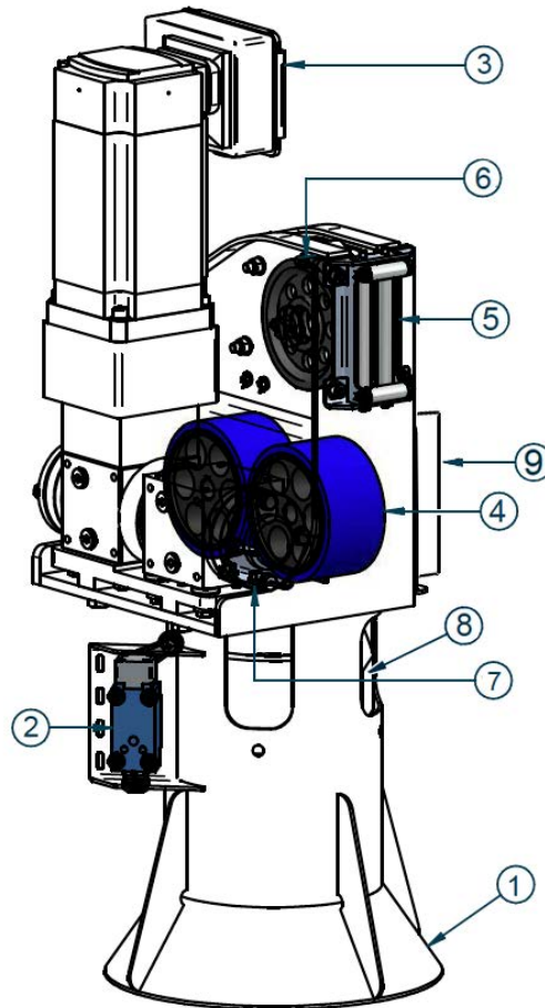
Sheave unit, transparent view
